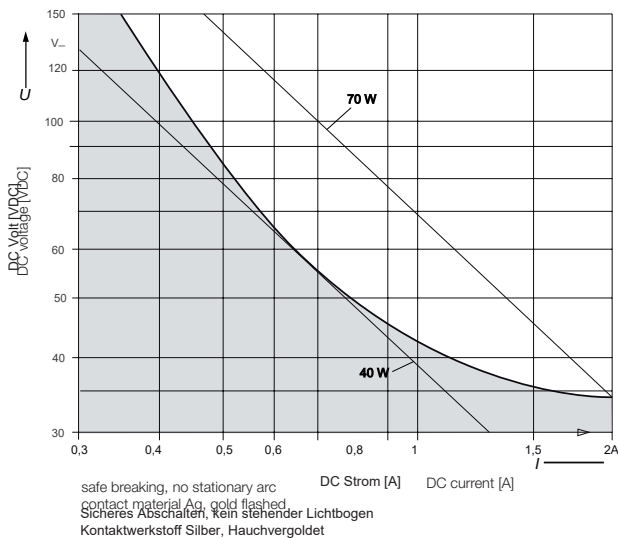
Max. DC Breaking capacity, contact sets B1xx, 61xx
