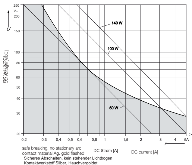
Max. DC Breaking capacity, contact sets F1xx
